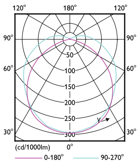
LEDForce WallPack
