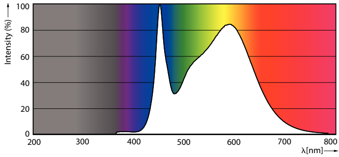
LEDTForce 60W WallPack EX39 840
