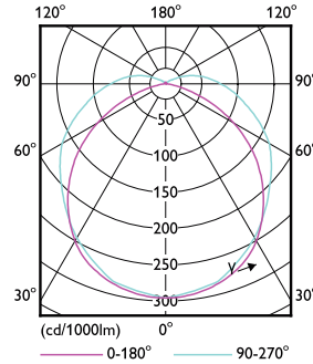
LEDTForce WallPack
