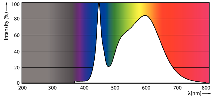
LEDTForce 115W Corncob EX39 840
