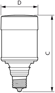
Corn lamp LED fan 115W EX39 840 CL
