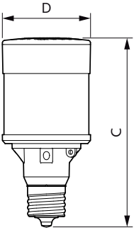
Corn lamp LED fan 80W EX39 850 CL
