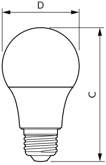
Bulb A60 120V 10-60W 800lm 5000K E26 ND
