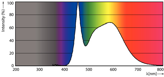
LEDbulb 9W E26 A9 850 FR
