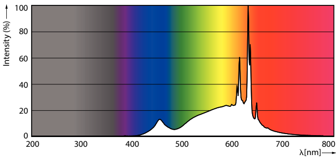
LEDbulb 16W A19 E26 922 927 FR
