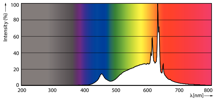
Bulb A19 120V 8.8-60W 800lm 2700K E26 D
