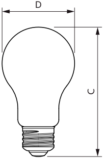
Bulb A19 120V 8.0-60W 800lm 5000K E26DCL
