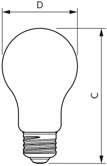
Bulb A19 120V 5.0-40W 450lm 5000K E26DCL
