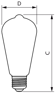
Bulb ST19 5-40W 350lm 2000K E26 D Amber
