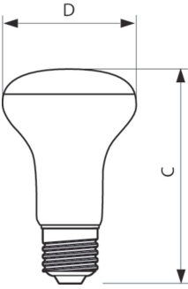
BR30 120V 19-120W 1200lm 2700K E26 D
