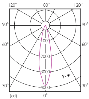
12-90W E26 PAR38 25D 827 2700K
