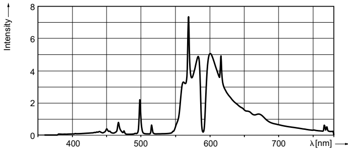
LDPB_SONHORTH_0001-Spectral power distribution B/W
