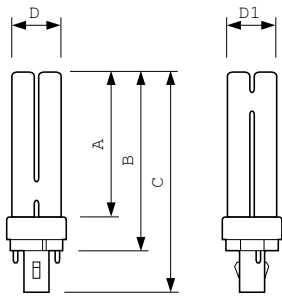
PL-C 18W/841/2P
