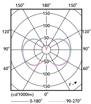
Light Distribution Diagram - 115CC/LED/840/LS EX39 G2 BB 277-480V 3/1
