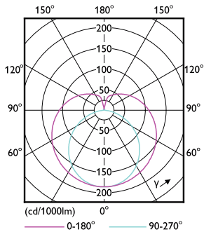
Light Distribution Diagram - 14T5HE/COR/46-840/MF21/G 25/1
