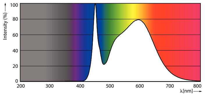
Spectral Power Distribution Colour - 14T5HE/COR/46-840/MF21/G 25/1
