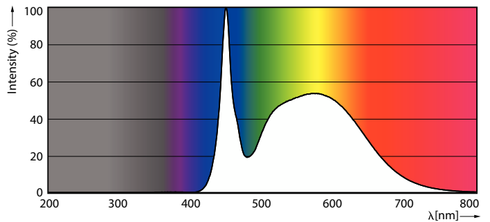
Spectral Power Distribution Colour - 10T5HE/COR/34-850/MF14/G 25/1
