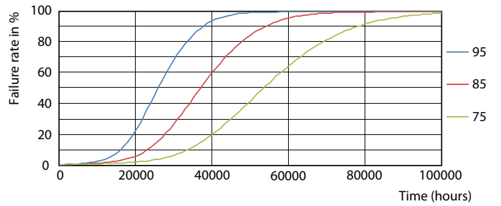
Life Expectancy Diagram - 25T5HO/COR/46-840/MF35/G 25/1
