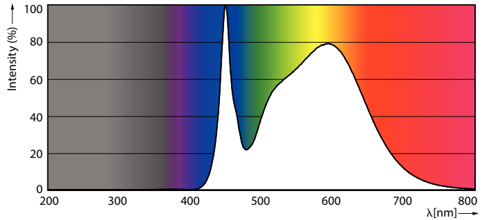
Spectral Power Distribution Colour - 25T5HO/COR/46-840/MF35/G 25/1
