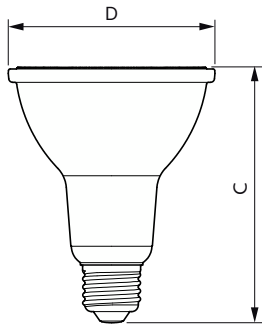
8.5PAR30L/LED/930/F25/DIM/GULW/T20 6/1FB
