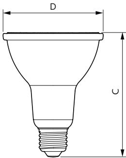
8.5PAR30L/LED/927/F25/DIM/GULW/T20 6/1FB
