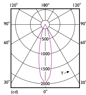
Light Distribution Diagram - 5.5PAR20/LED/F25/940/DIM/G/T20 6/1FB
