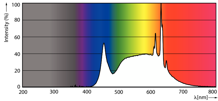
Spectral Power Distribution Colour - 5.5PAR20/LED/F25/940/DIM/G/T20 6/1FB
