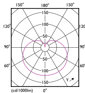
Light Distribution Diagram - 8.8A19/LED/930/FR/P/E26/ND/T20 6/1FB
