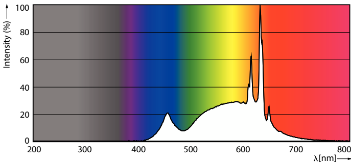
Spectral Power Distribution Colour - 8.8A19/LED/930/FR/P/E26/ND/T20 6/1FB
