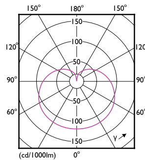
Light Distribution Diagram - 5A19/LED/950/FR/P/E26/ND/T20 6/1FB
