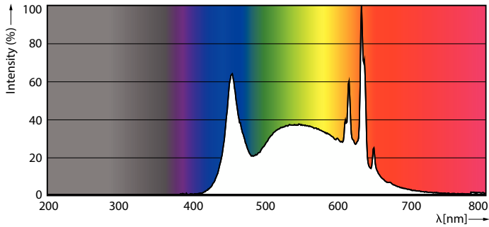
Spectral Power Distribution Colour - 5A19/LED/950/FR/P/E26/ND/T20 6/1FB
