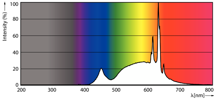
Spectral Power Distribution Colour - 5A19/LED/930/FR/P/E26/ND/T20 6/1FB
