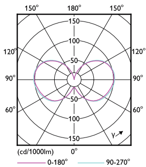
LEDForce LS EX39 63W Corncob EX39-LDD
