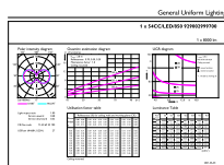
Light Distribution Diagram - 54CC/LED/850/LS EX39 G3 BB 3/1
