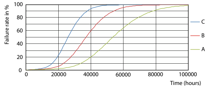
Life Expectancy Diagram - 15.5T8/COR/48-850/MF21/G/BAA 25/1
