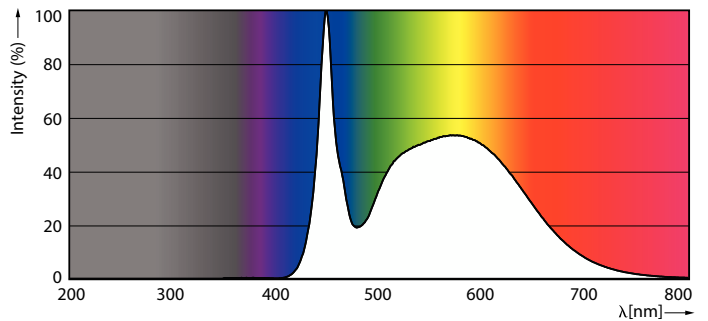
Spectral Power Distribution Colour - 15.5T8/COR/48-850/MF21/G/BAA 25/1
