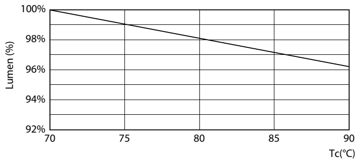
Lumen Maintenance Diagram - 15.5T8/COR/48-850/MF21/G/BAA 25/1
