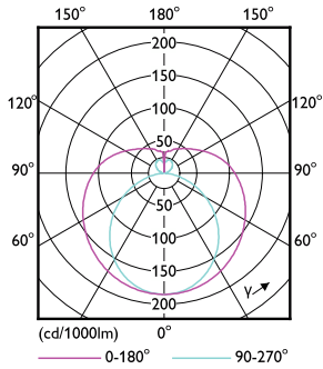
Light Distribution Diagram - 15.5T8/COR/48-850/MF21/G/BAA 25/1
