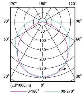
LEDForce WallPack
