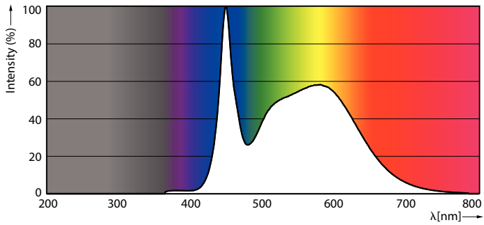
LEDForce 45W Corncob EX39 850
