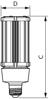
Corn lamp LED Gen2 27W E26 840 CL
