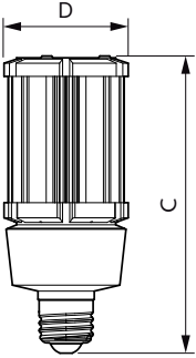
Corn lamp LED Gen2 18W E26 850 CL
