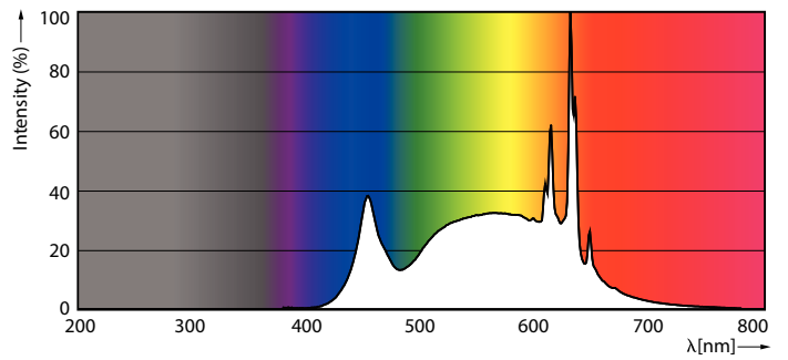
LEDbulb 16W A19 E26 940 FR
