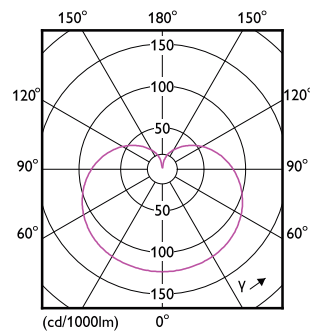
Light Distribution Diagram - 12.2A19/PER/927/P/E26/DIM 6/1FB T20
