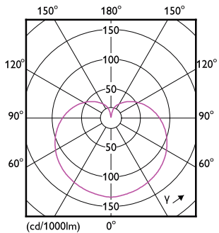
LEDbulb A19 E26 800lm FR
