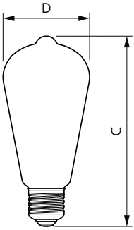
ST19 5.5-60W 500lm 2700-2200K E26 D CL
