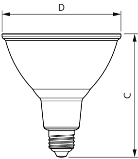
PAR38 13-120W 1200lm 25D 3000K E26 D
