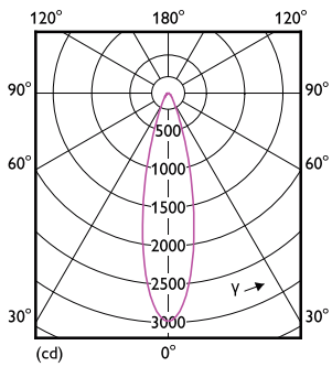
LEDspots 9,4W PAR30S E26 930 25D
