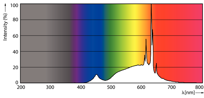
LEDBulbs_R20 120V 5-45W 450lm 90D 2700-2200K E26
