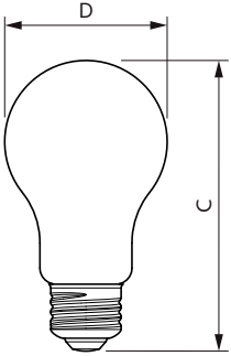
Bulb A19 120V 5.5-40W 450lm 2200-2700K
