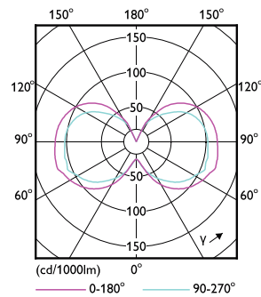
LEDcapsule 3,6W G9
