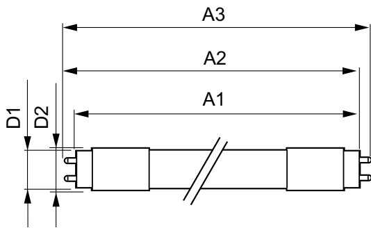
TLED 1200mm HFV16-28W 2100lm 4000K ND
