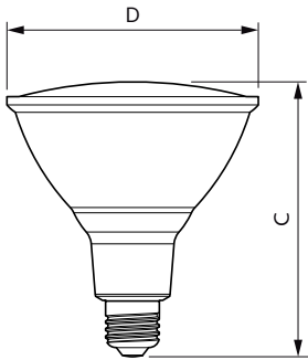
13.5PAR38/PER/BLUE/ND/ULW/G/120V 4/1FB
