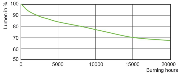
Lumen Maintenance Diagram - CDM145/U/O/4K/ED28 EA ALLSTART
