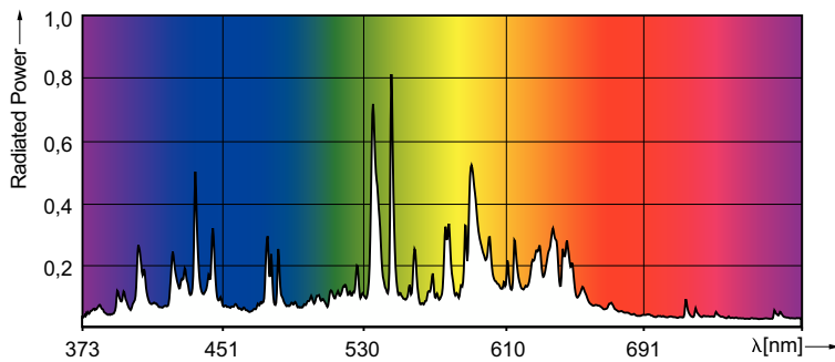
Spectral Power Distribution Colour - CDM145/U/O/4K/ED28 EA ALLSTART
