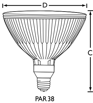
CDM 100W/830 E26 PAR38 FL 25D ALTO Elite
