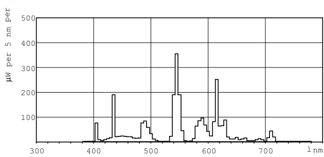
LDPB_TL5ECO_835-Spectral power distribution B/W
