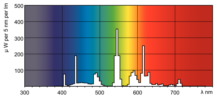
LDPO_TL5HEECO_835-Spectral power distribution Colour
