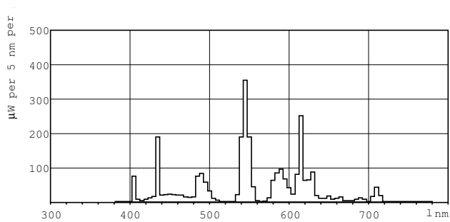
LDPB_TL5HEECO_835-Spectral power distribution B/W
