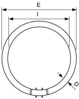
TL5-C 55W/830
