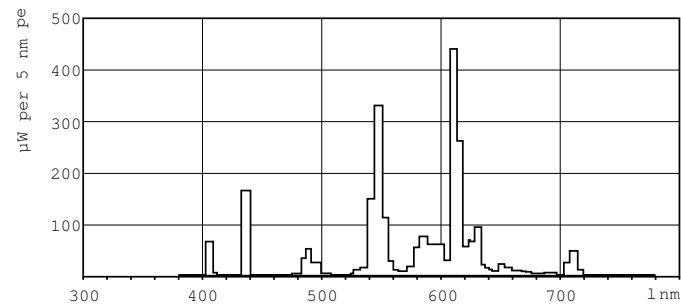
LDPB_PLTTOP4P_827-Spectral power distribution B/W
