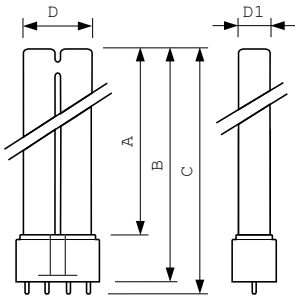
PL-L 36W/830/4P
